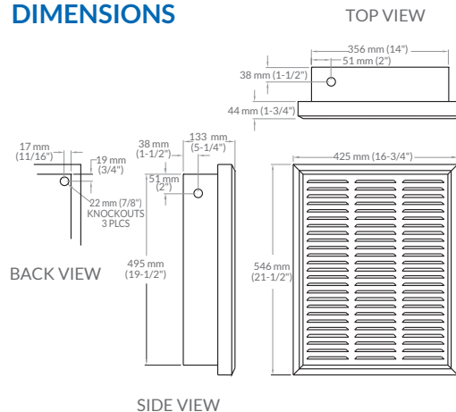
RFITF T-bar Ceiling Mount Trim (white only)
